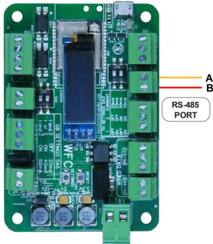
WFC communicator
