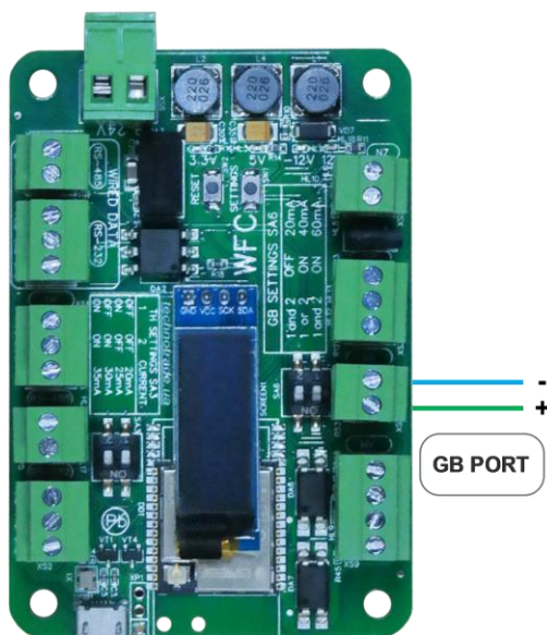
WFC communicator
