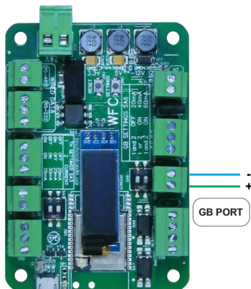
WFC communicator
