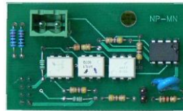
Nuovo Pignone interface boards for RS-485 interface for monoproduct and multiproducts dispensers
