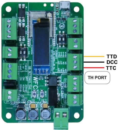
WFC communicator
