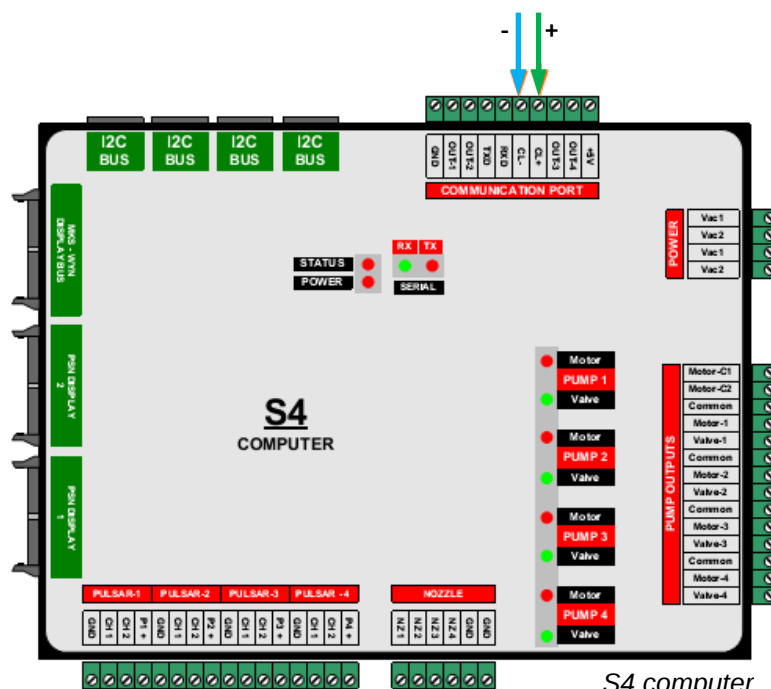
S4 computer
