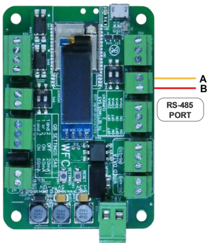
WFC communicator
