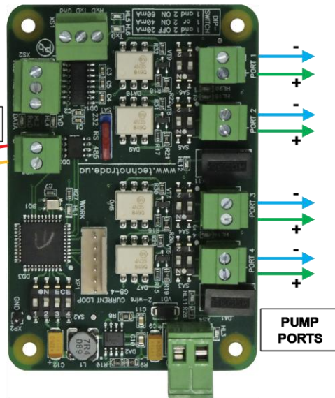
GB-4 interface converter
