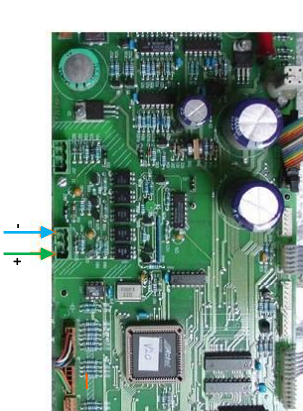
Batchen dispenser board
